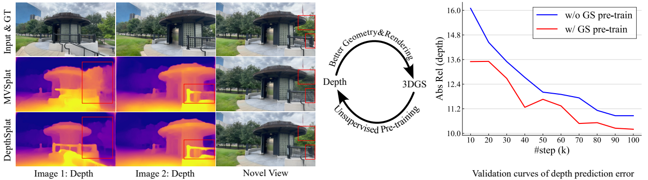
Figure 1. DepthSplat enables cross-task interactions between Gaussian splatting and depth. Left: Better depth leads to improved Gaussian splatting reconstruction. Right: Unsupervised depth pre-training with Gaussian splatting leads to reduced depth prediction error.
