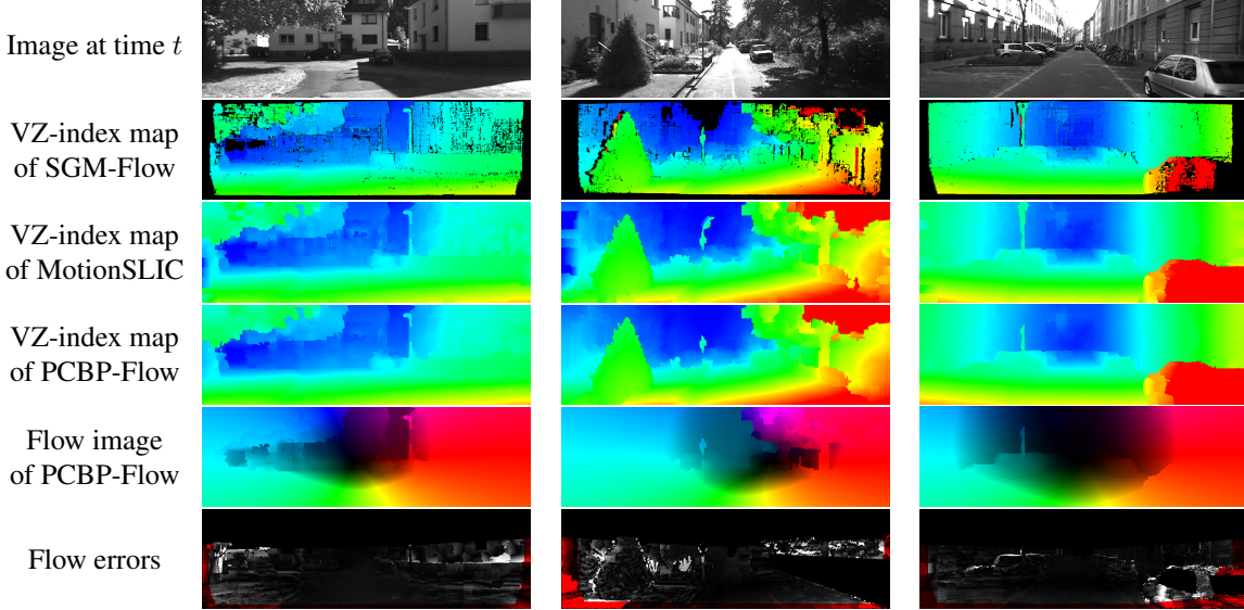
Figure 3. KITTI examples
