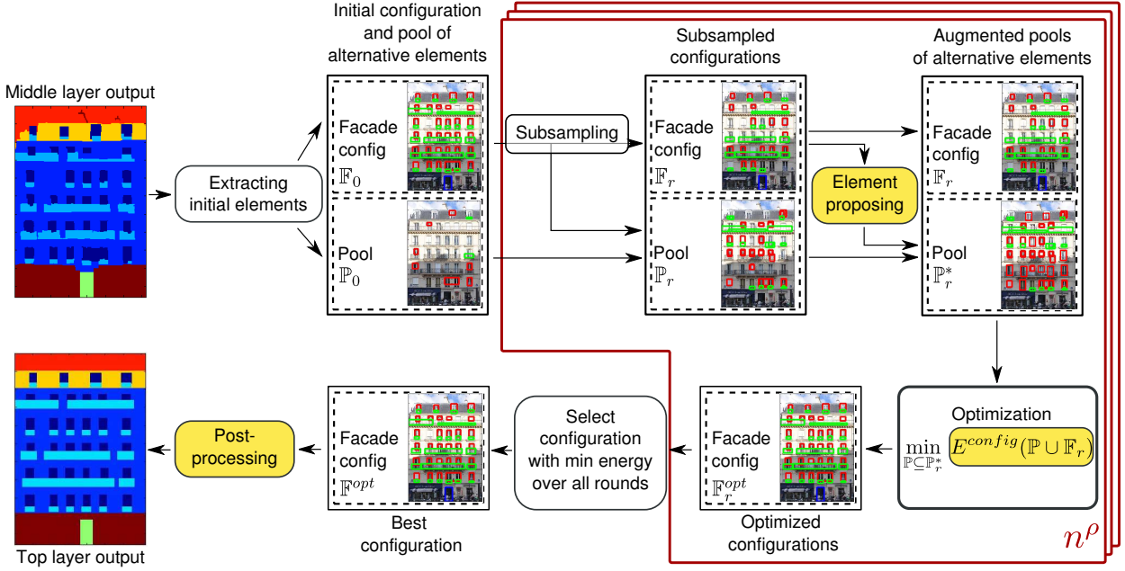
Fig. 10 A high-level overview of the top layer. The blocks highlighted in yellow depend on weak architectural principles, see text for description.
