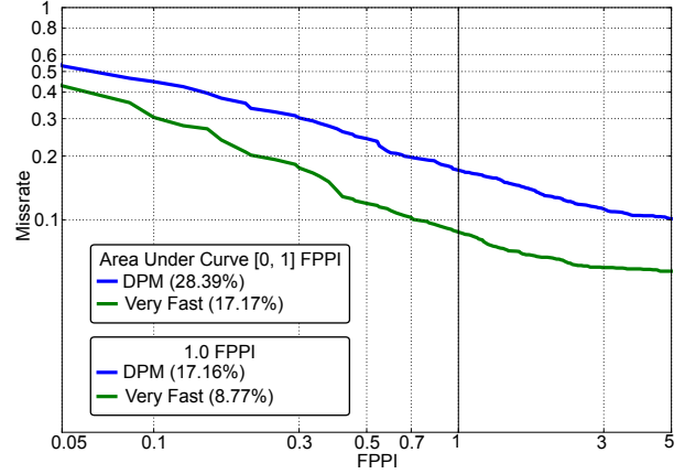
Fig. 5 Comparison of the dataset-specific DPM and Very Fast on the task of window detection. The plot shows the mean false positive per image (FPPI) versus miss-rate, averaged over 5 folds.
