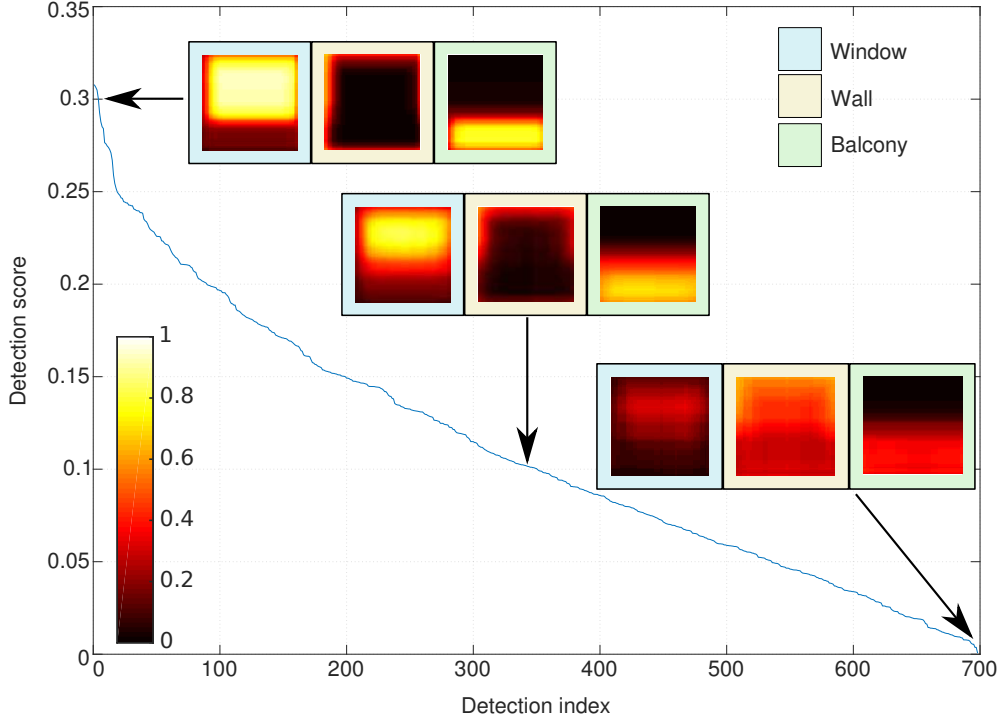
Fig. 8 (Best viewed in color) Learning label distributions for the window detector. Window detections on the ECP validation set are sorted by their score in descending order. High-scoring detections (top-left) provide a much stronger prior than the low-scoring detections (bottom-right)
