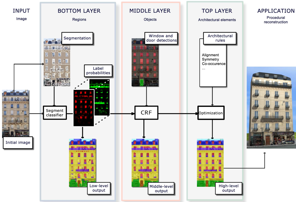
Fig. 2 The proposed three-layered approach to facade parsing.
