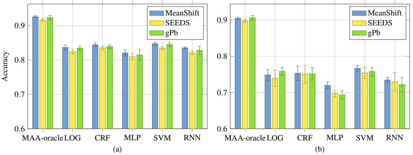
Fig. 3 (a) Pixel-wise and (b) class-wise accuracy of different segmentation algorithms and classifiers on the ECP dataset. The results are calculated as the mean, and error bars as the standard deviation of results calculated from five cross-validation folds.
