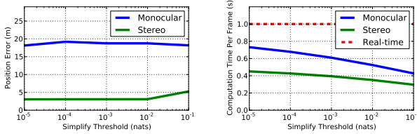
Fig. 6. Simplification Threshold: Impact of the simplification threshold \epsilon on localization accuracy (left) and computation time (right). See Section 4.4.
