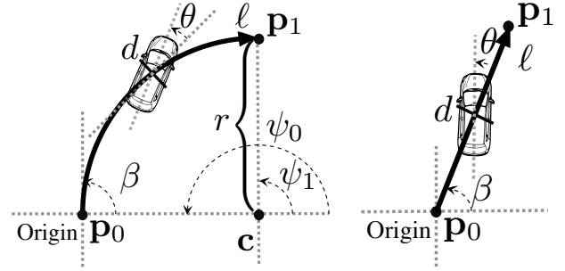
Fig. 3. Street Segment: Each street segment has a start and end position p_0 and p_1 , a length \ell , an initial heading of the street segment \beta and a curvature parameter \alpha = \frac{\psi_1 - \psi_0}{\ell} . For arc segments c is the circle center, r is the radius and \psi_0 and \psi_1 are the start and end angles of the arc. For linear segments, \alpha = 0 .
