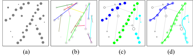
Figure 1. Given a number of unlabeled object detections (a) and a number of possible trajectory hypotheses (b), our method labels all detections (c) and re-estimates the trajectories (d) using an alternating discrete-continuous optimization scheme.
