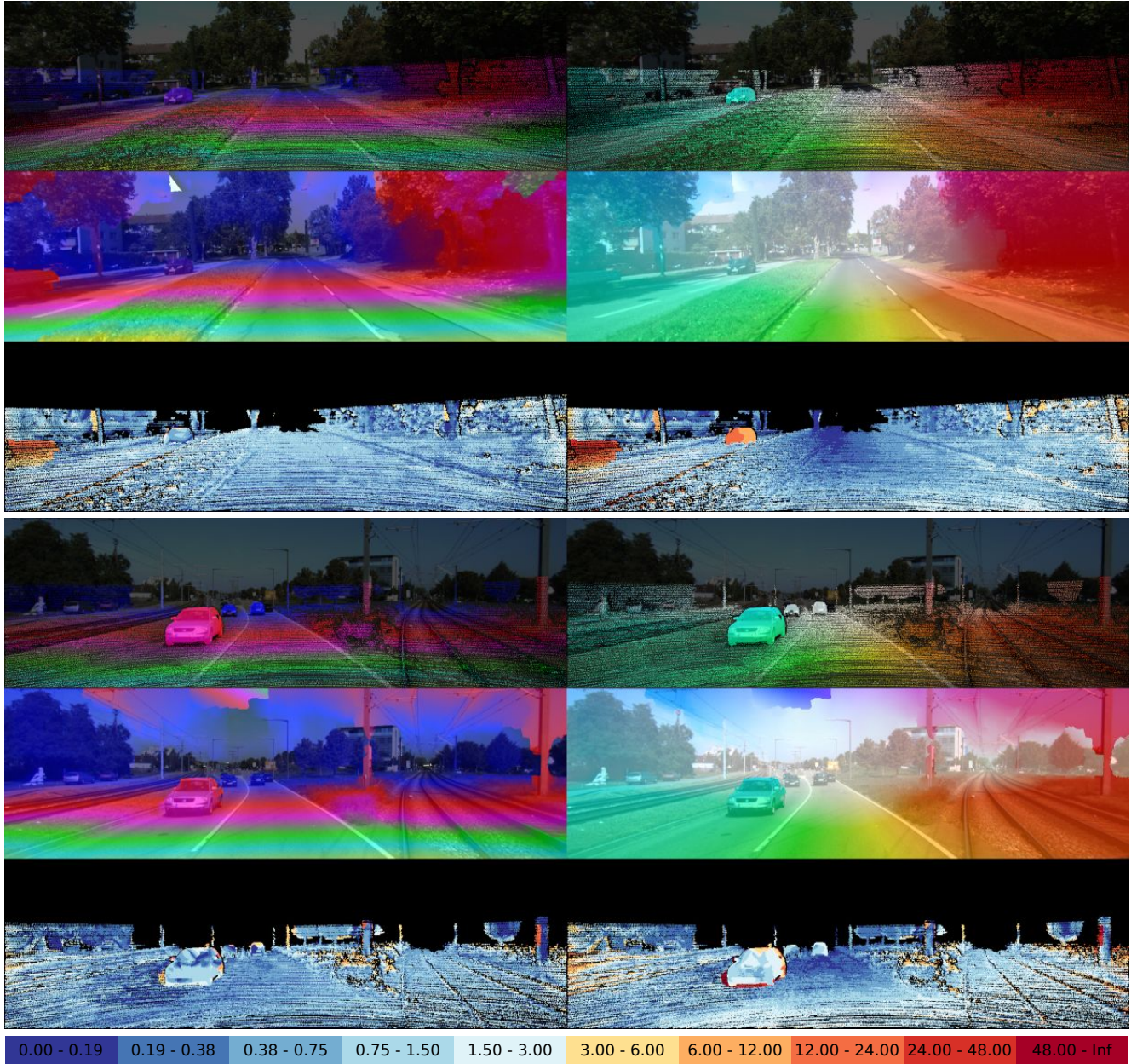
Figure 8: Qualitative Results. Each subfigure shows from top-to-bottom: The disparity and optical flow ground truth in the reference view, the disparity map (D1) and optical flow map (F1) estimated by our scene flow algorithm, and the respective error images using the color scheme depicted in the legend.
