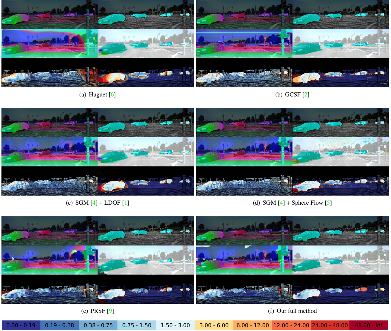
Figure 33: Comparison of Results. Each subfigure shows from top-to-bottom: The disparity and optical flow ground truth in the reference view, the disparity map (D1) and optical flow map (FI) estimated by the specified algorithm, and the respective error images using the color scheme depicted in the legend.
