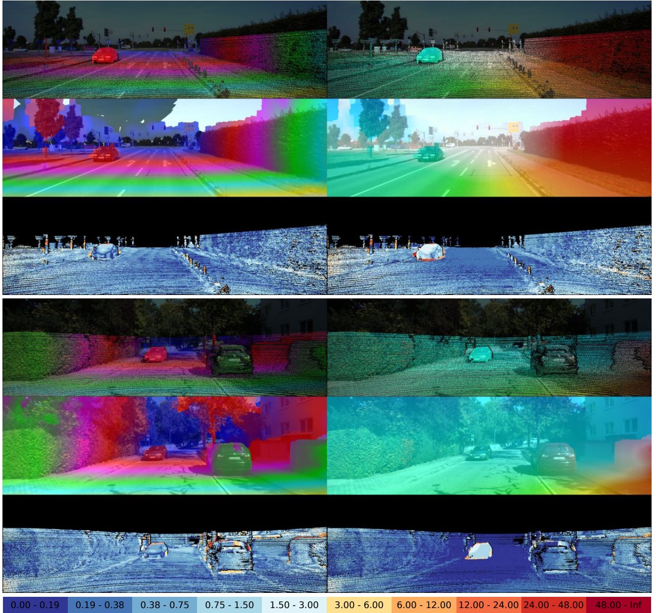
Figure 15: Qualitative Results. Each subfigure shows from top-to-bottom: The disparity and optical flow ground truth in the reference view, the disparity map (D1) and optical flow map (F1) estimated by our scene flow algorithm, and the respective error images using the color scheme depicted in the legend.
