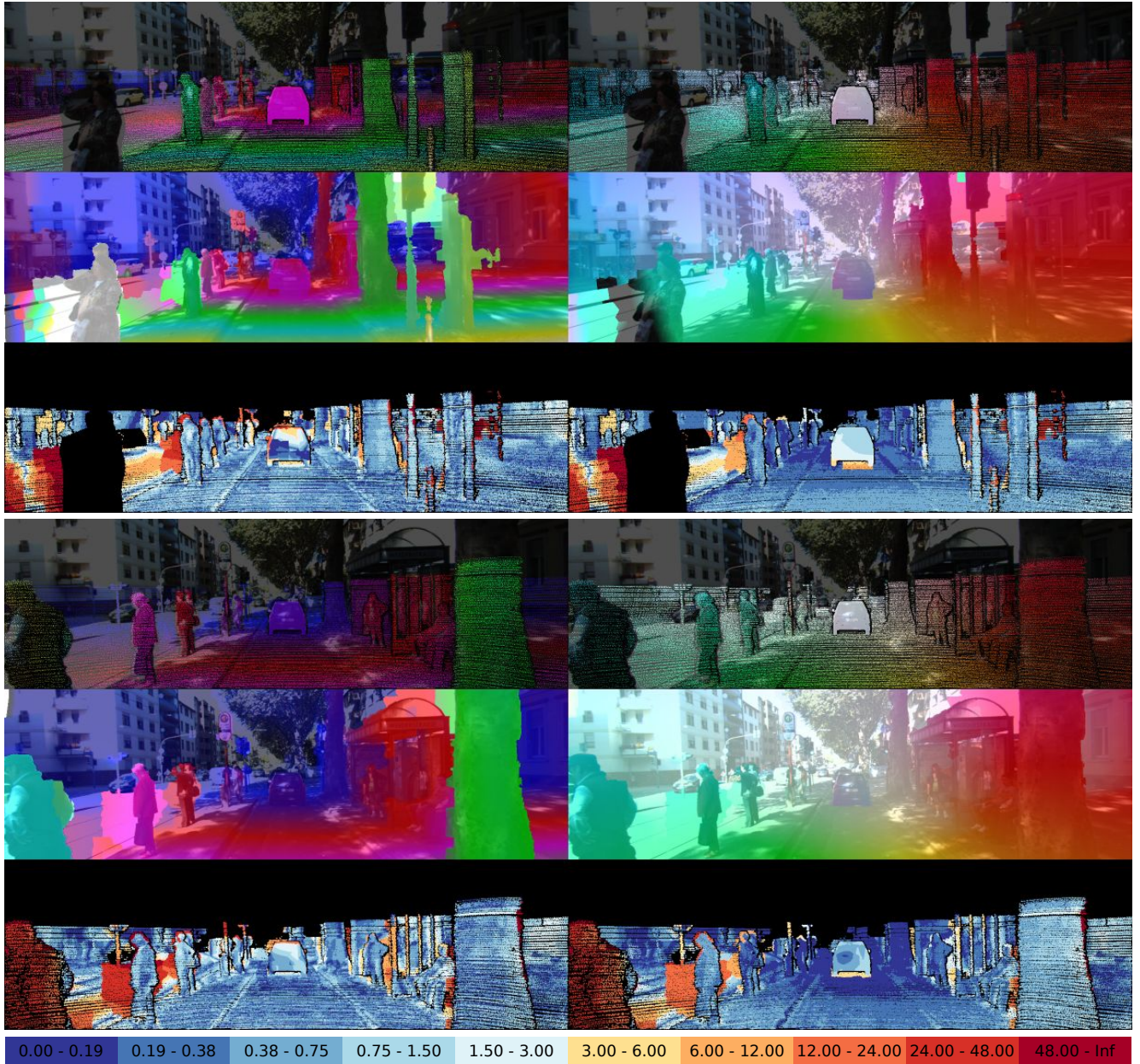
Figure 26: Qualitative Results. Each subfigure shows from top-to-bottom: The disparity and optical flow ground truth in the reference view, the disparity map (D1) and optical flow map (F1) estimated by our scene flow algorithm, and the respective error images using the color scheme depicted in the legend.
