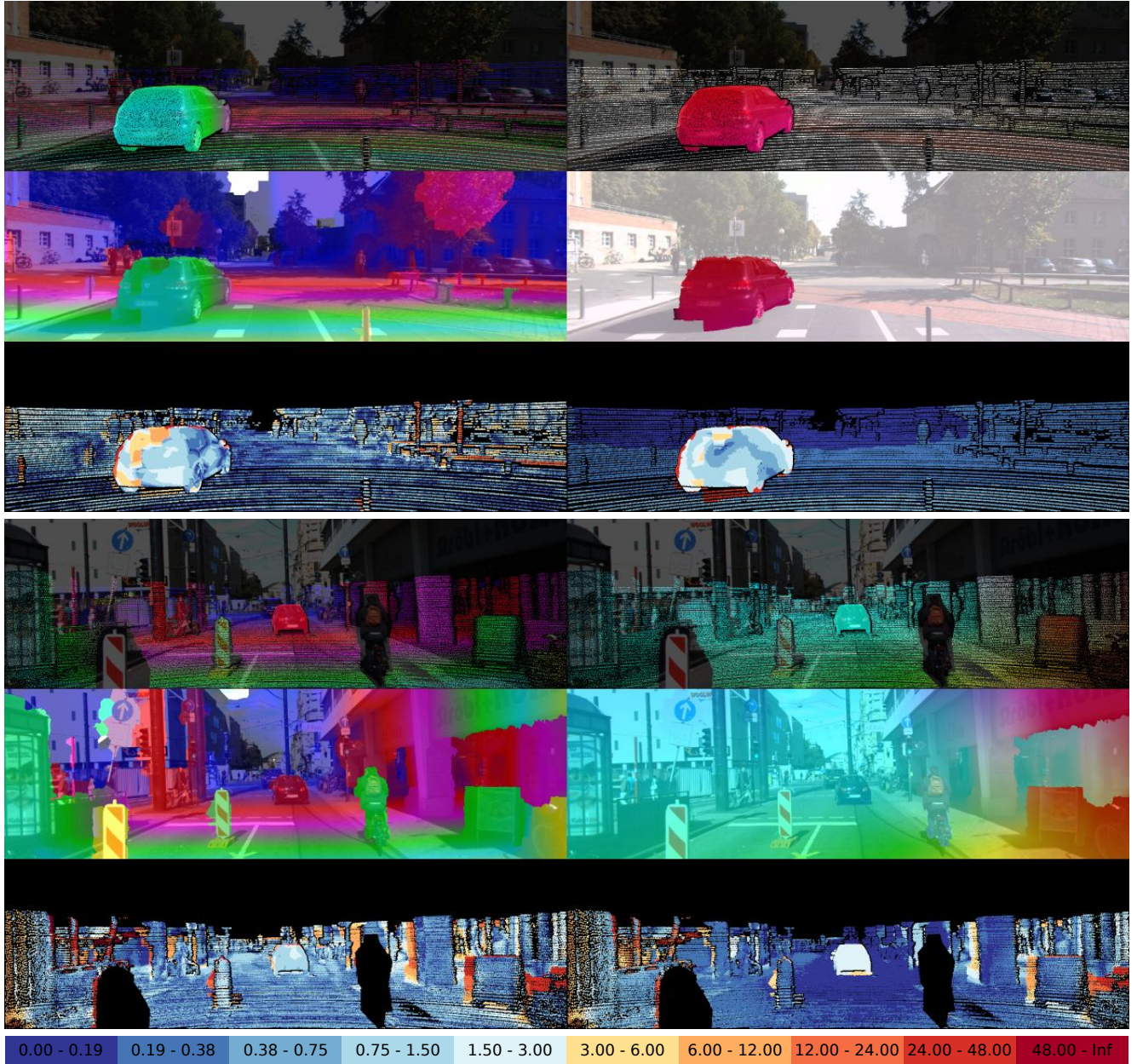
Figure 25: Qualitative Results. Each subfigure shows from top-to-bottom: The disparity and optical flow ground truth in the reference view, the disparity map (D1) and optical flow map (F1) estimated by our scene flow algorithm, and the respective error images using the color scheme depicted in the legend.
