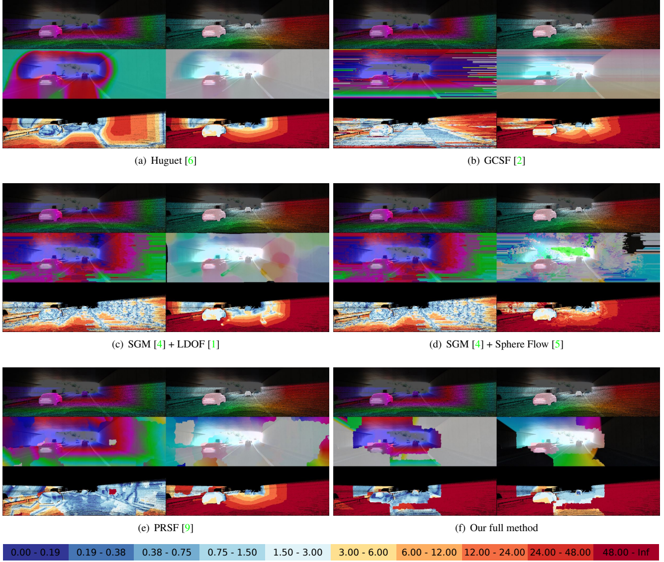
Figure 35: Comparison of Results. Each subfigure shows from top-to-bottom: The disparity and optical flow ground truth in the reference view, the disparity map (D1) and optical flow map (FI) estimated by the specified algorithm, and the respective error images using the color scheme depicted in the legend.
