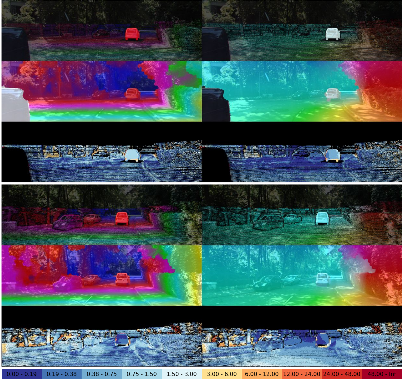
Figure 9: Qualitative Results. Each subfigure shows from top-to-bottom: The disparity and optical flow ground truth in the reference view, the disparity map (D1) and optical flow map (F1) estimated by our scene flow algorithm, and the respective error images using the color scheme depicted in the legend.
