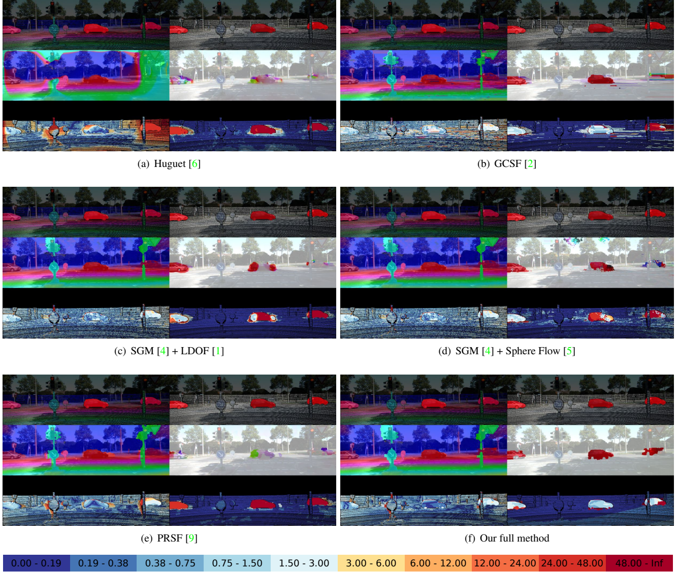
Figure 32: Comparison of Results. Each subfigure shows from top-to-bottom: The disparity and optical flow ground truth in the reference view, the disparity map (D1) and optical flow map (F1) estimated by the specified algorithm, and the respective error images using the color scheme depicted in the legend.
