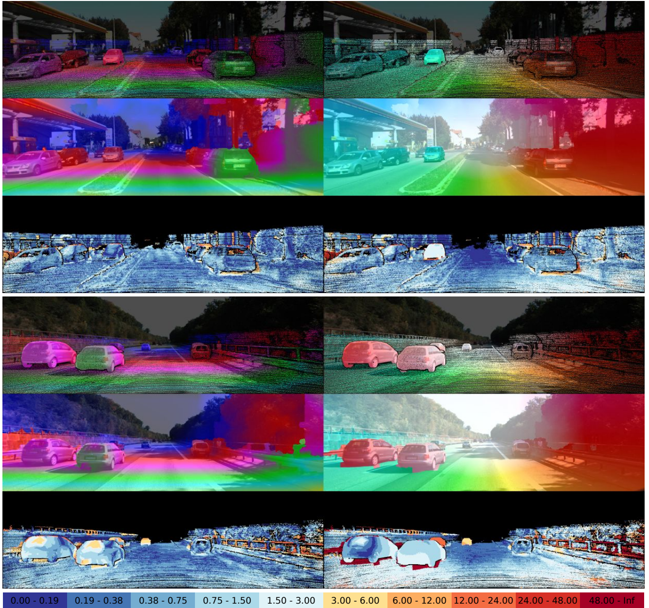
Figure 28: Qualitative Results. Each subfigure shows from top-to-bottom: The disparity and optical flow ground truth in the reference view, the disparity map (D1) and optical flow map (F1) estimated by our scene flow algorithm, and the respective error images using the color scheme depicted in the legend.
