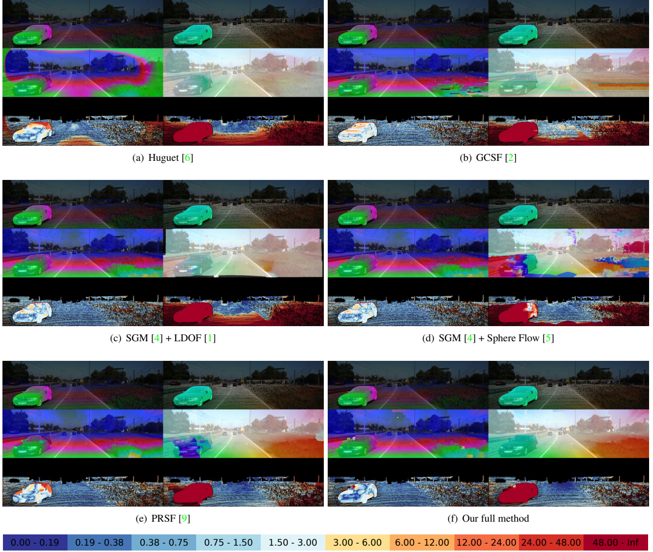
Figure 36: Comparison of Results. Each subfigure shows from top-to-bottom: The disparity and optical flow ground truth in the reference view, the disparity map (D1) and optical flow map (F1) estimated by the specified algorithm, and the respective error images using the color scheme depicted in the legend.
