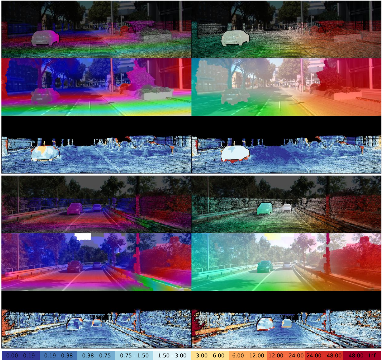
Figure 27: Qualitative Results. Each subfigure shows from top-to-bottom: The disparity and optical flow ground truth in the reference view, the disparity map (D1) and optical flow map (F1) estimated by our scene flow algorithm, and the respective error images using the color scheme depicted in the legend.
