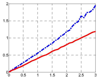
Fig. 4 The reprojection error vs. the noise level with the linear minimization (dashed line in blue) and after the non-linear refinement (solid line in red). Both units are in pixels.
