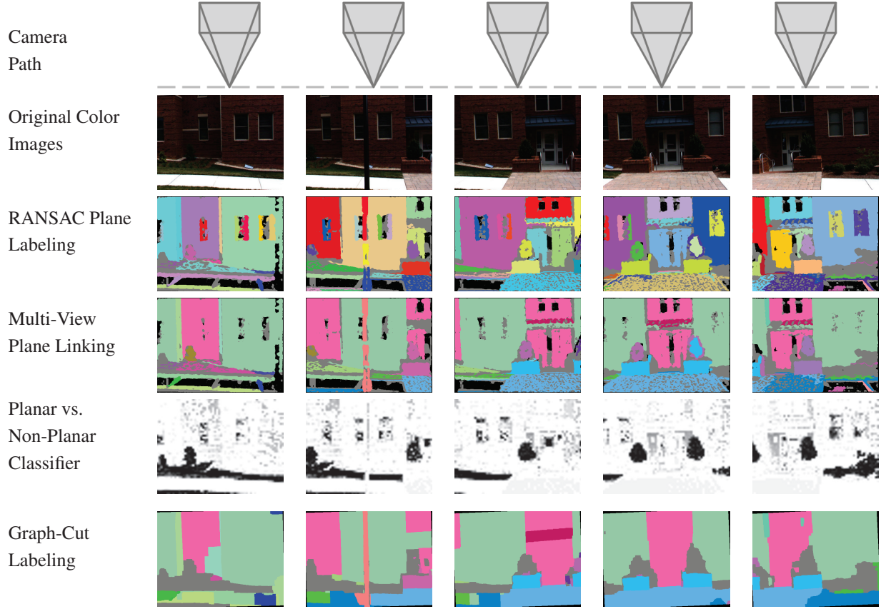
Figure 3. The second row shows a subset of the images used to compute the depth maps. The third row illustrates the plane detection results of our modified RANSAC technique. The fourth row shows the plane labels after linking. Note that the same scene plane now has a consistent label. The fifth row shows the classification results of the image into planar or non-planar structure (planar class probability black=0, white=1). The sixth row shows the results of the graph cut based plane assignment. See Figure 6 for the resulting 3D model.
